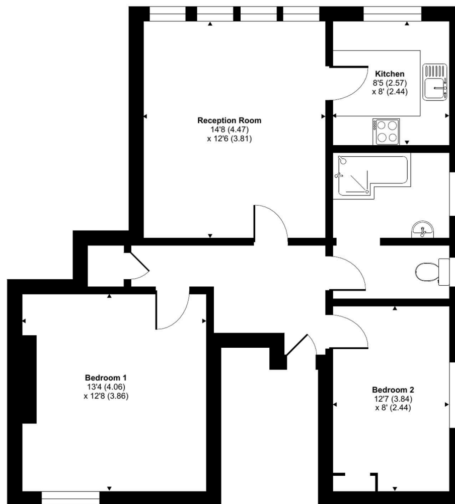
SECOND FLOOR
